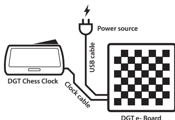
Figure 1. Recording set-up.
